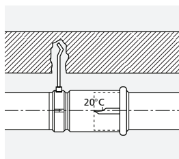
Horizontal assembly (e.g. at an ambient temperature of 20°C).
