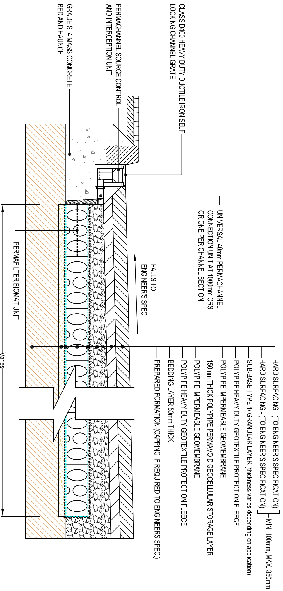
TYPICAL SECTION THROUGH POLYPYPE PERMACHANNEL AND PERMAVOID ATTENUATION TANK Scale (1:15)
