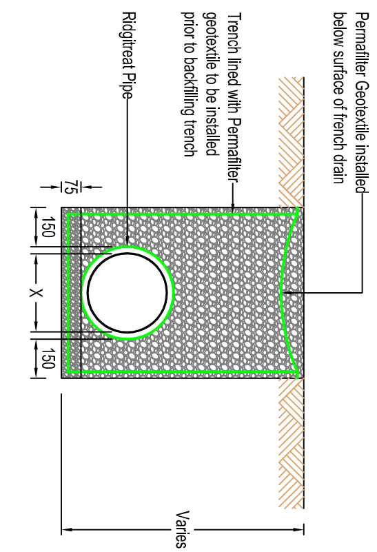
French Drain (Infiltration) installed with Ridgitreat and enclosed with Permafilter Geotextile Scale (1:20)
